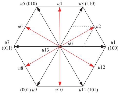
Fig. 16. Auxiliary voltage vector MPC ( N = 6 ).
