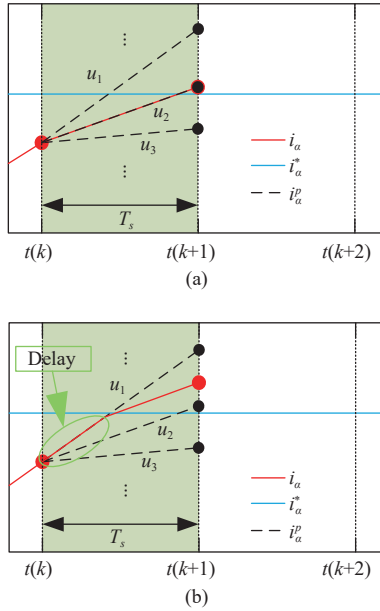
Fig. 17. Model predictive current control. (a) Without delay; (b) With delay.
