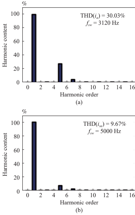
Fig. 12. Frequency spectra of the phase current i_a at 600 rpm with 4 N·m load using (a) conventional MPTC and (b) proposed MPTC [51].
