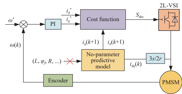
Fig. 7. Block diagram of FCS-MPC applied to PMSM based on no-parameter predictive model.
