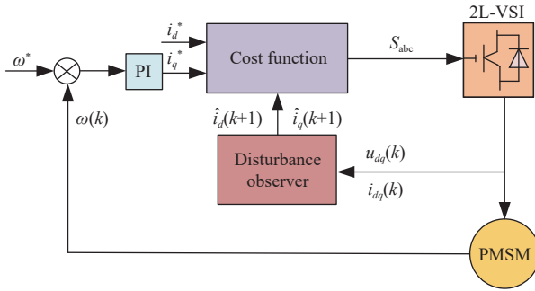
Fig. 6. Block diagram of FCS-MPC applied to PMSM based on observer estimation and compensation.
