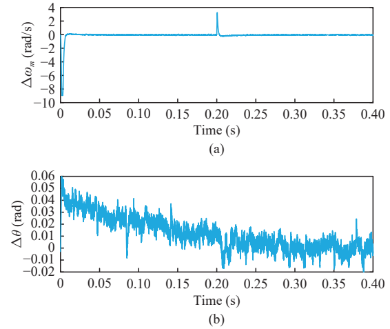
Fig. 22. The FCS-MPC with FPS-PLL. (a) Angular velocity tracking error; and (b) Angle tracking error [161].
