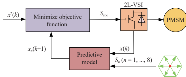
Fig. 4. A typical MPC block diagram for PMSMs.
