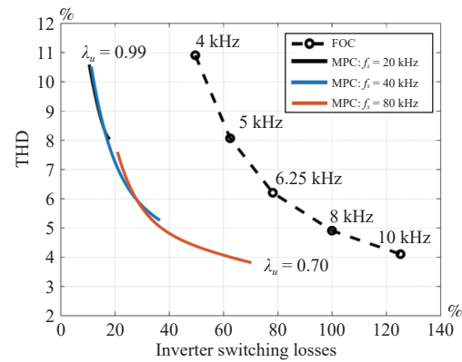
Fig. 19. The relationship between inverter switching loss and THD [56].
