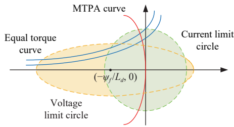
Fig. 18. The trajectory of maximum torque per ampere (MTPA) in [139].
