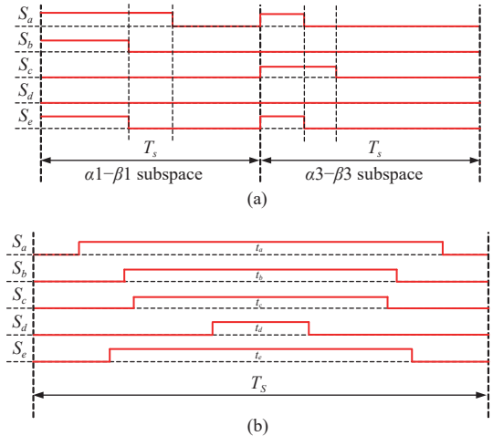
Fig. 11. Pulse generation. (a) Original switching signal; (b) Rearranged fixed switching frequency signal.
