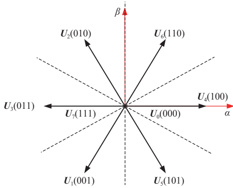
Fig. 3. Voltage vectors space of 2L-VSI.
