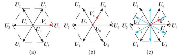
Fig. 14. Voltage vector diagram. (a) Conventional FCS-MPC; (b) Duty cycle FCS-MPC; (c) FCS-MPC based on a hybrid control set.
