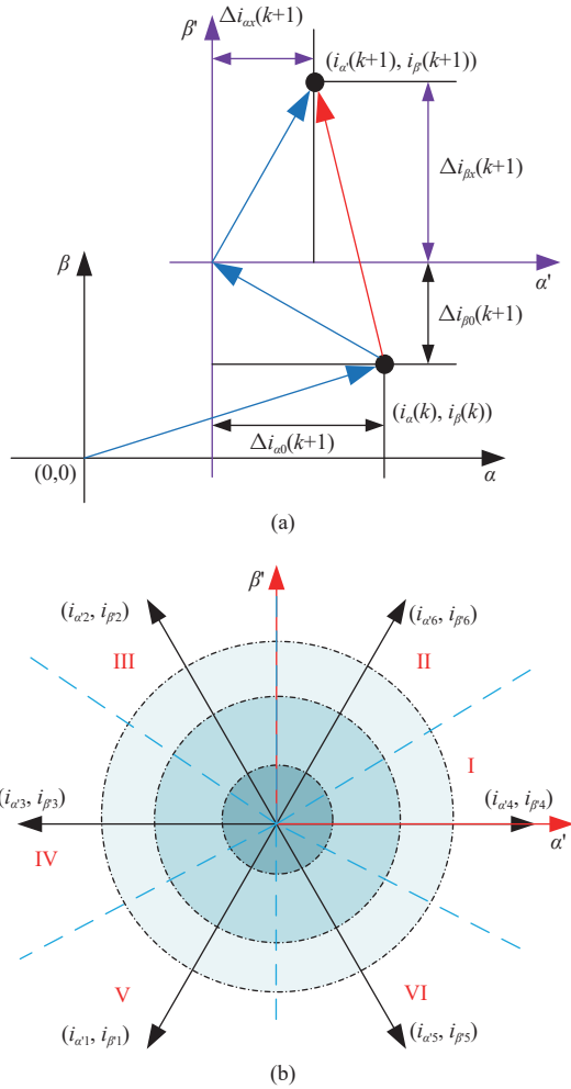
Fig. 10. The new reference frame of [24]. (a) New reference frame \alpha' - \beta' based on stator reference frame \alpha - \beta . (b) The current loci when different active voltage vectors are applied in the reference frame \alpha' - \beta' .
