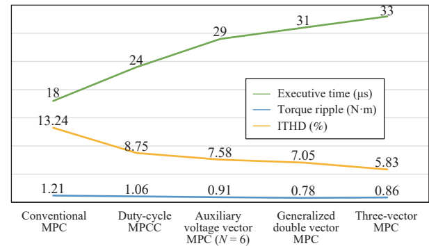
Fig. 15. Execution time, current harmonics and torque ripple under various control schemes.
