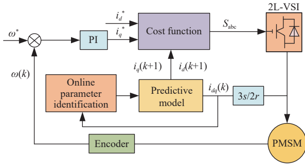
Fig. 8. Block diagram of FCS-MPC applied to PMSM based on online parameter identification.
