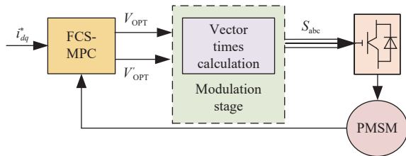
Fig. 13. The control diagram of a conventional M2PC for PMSMs [117].
