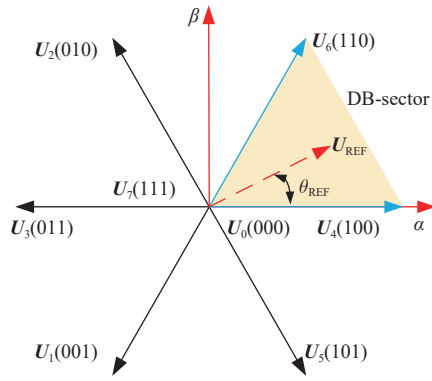
Fig. 9. 2L-VSI's deadbeat search solution.
