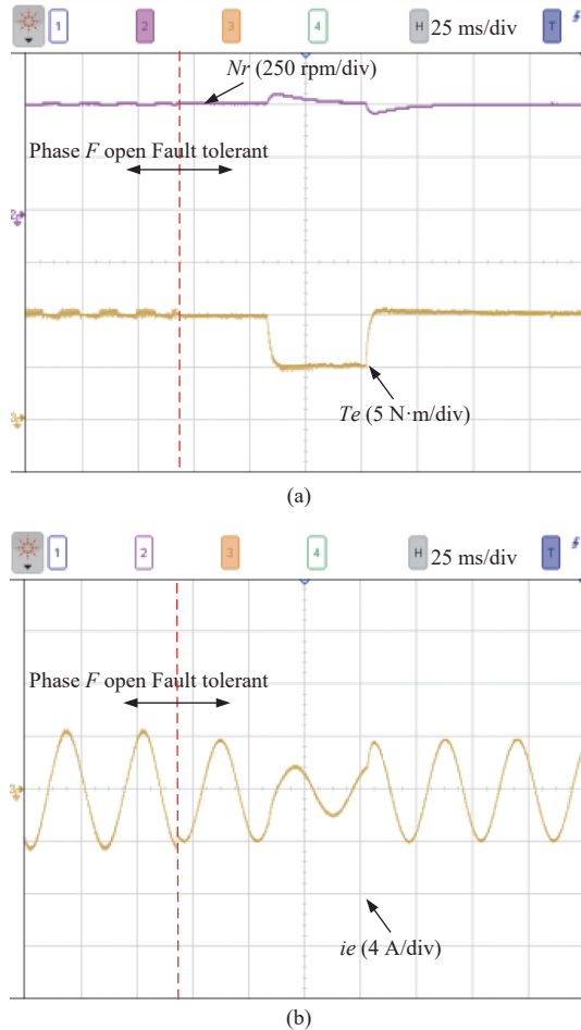
Fig. 21. Load torque variation test based on MPCC fault-tolerant control. (a) Torque and speed; and (b) E-phase current. [160].
